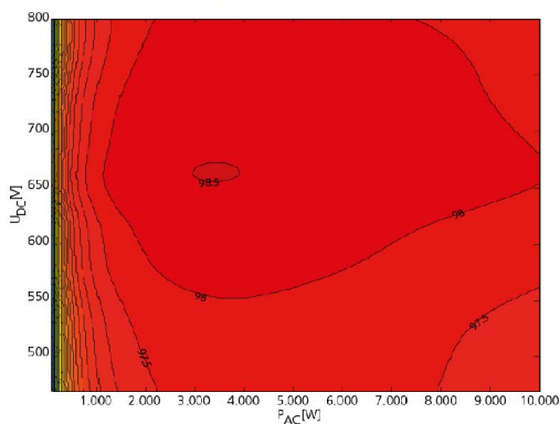
3D efficiency diagram for blueplanet 10.0 TL3
