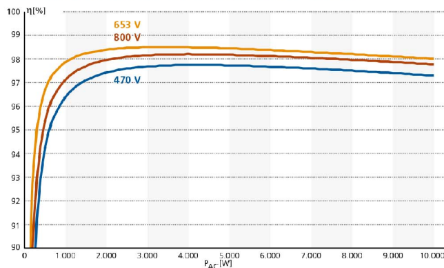
Efficiency characteristic curve for blueplanet 10.0 TL3
